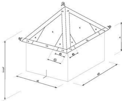
11. Pyramidedak
